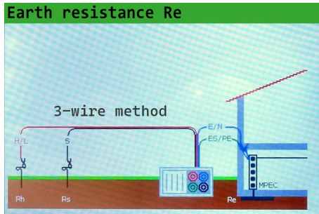
Fig. 8: Earth Resistance Measurement R_e , Wiring and Results
