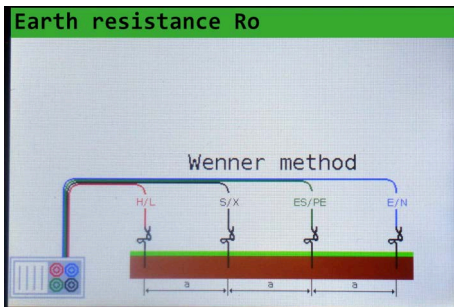
Fig. 9: Earth Resistance Measurement R_0 , Wiring and Results
