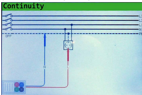
Fig. 7: Continuity Test, Wiring and Results
