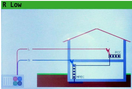
Fig. 6: R Low Test, Wiring and Results
