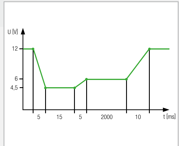
Simulation of a starter motor characteristic curve
