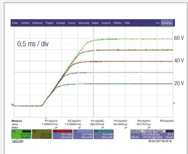
Rise time of output power
