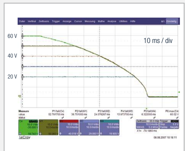
Fall time of output power
